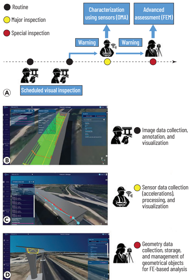
Figure 7. Different twin inspection applications for existing bridges during their lifecycle: (a) multilevel inspection workflow, progressing from routine visual inspection through sensor-based characterization to advanced FEM assessment when triggered by warnings; (b-d) data collection at the three inspection levels.
