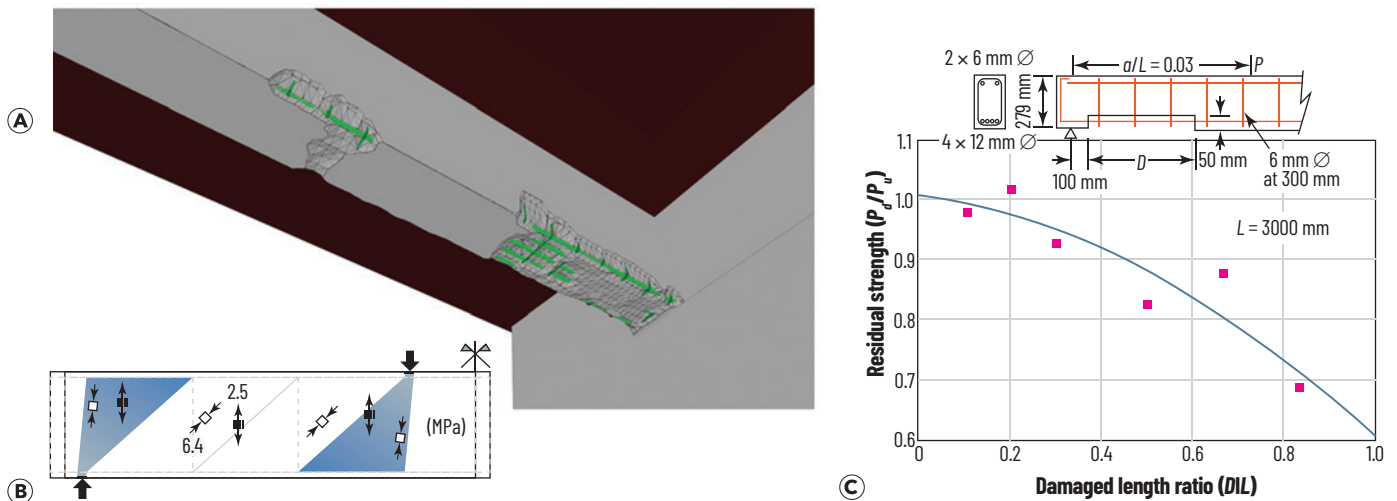
Figure 4. Spalling damage and its structural consequences: (a) photogrammetric recording subtracted from the bridge 3D model; (b) disrupted load path from loss of reinforcement bond, shown as a stress field; (c) resulting reduction in structural resistance (Raoof and Lin 1997).
