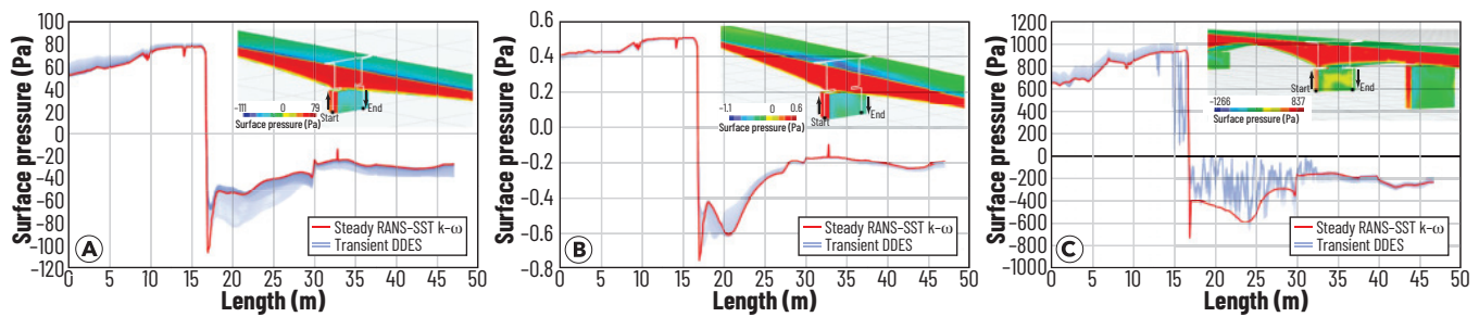
Figure 13. Surface pressure distribution along the probe line for three loading scenarios, based on 60-time steps ( \Delta t = 0.5 s). Results compare steady RANS (SST k-\omega ) and transient DDES simulations (Kazemian et al. 2023): (a) extreme wind condition; (b) extreme cold condition; (c) wind design values corresponding to a 3000-year return period.
