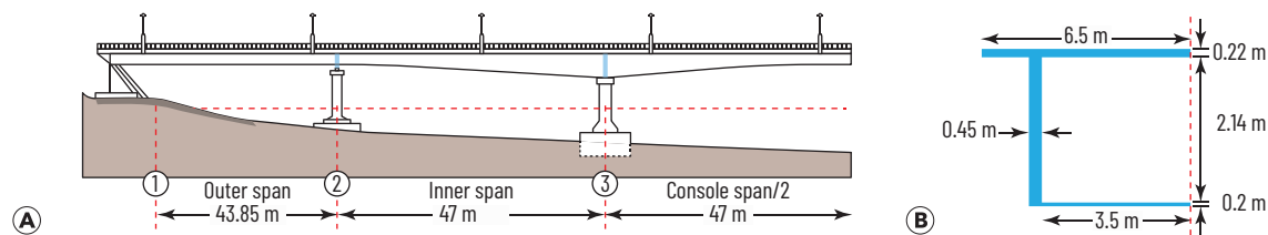
Figure 11. The Kalix Bridge: (a) overall structural geometry and span lengths; (b) representative cross-section of the prestressed concrete girder (reproduced from Sas et al. 2024).
