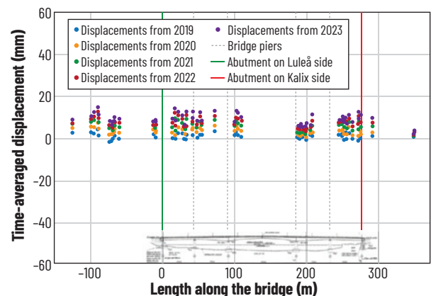
Figure 12. Vertical displacement trends of the Kalix Bridge over the observation period (2019–2023), obtained from satellite-based Interferometric Synthetic Aperture Radar (InSAR). Displacements are shown as a function of position along the bridge; data are filtered to include only points with coherence > 0.65 (Zandi and Malekloo 2025).
